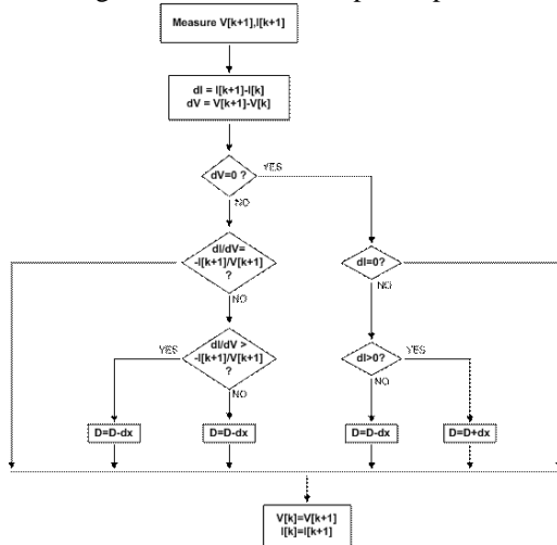
Figure 6. The Method of Incremental Conductance
