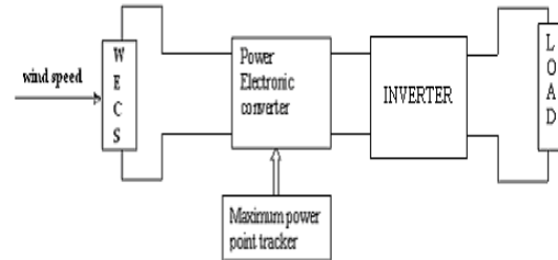
Figure 2: Block Diagram for Maximum Power Point Tracking
