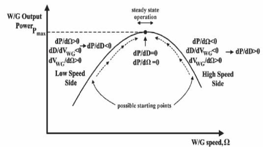
Figure 4.MPP tracking process.
