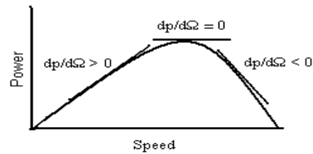
Figure 3: Probable Displacement of the Operating Point
