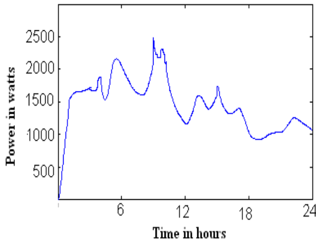
Figure 12. Power output using IC method (Variable load)
