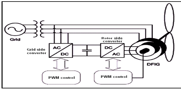
Figure 1: Conversion System of Wind Energy
