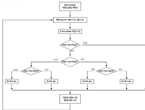
Figure 5. Method of Perturbation and Observation
