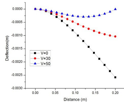
Fig 6: Cantilever lamination and its Centerline deflection [p/-45/45] as under uniform loading and input voltages of diverse actuators.
