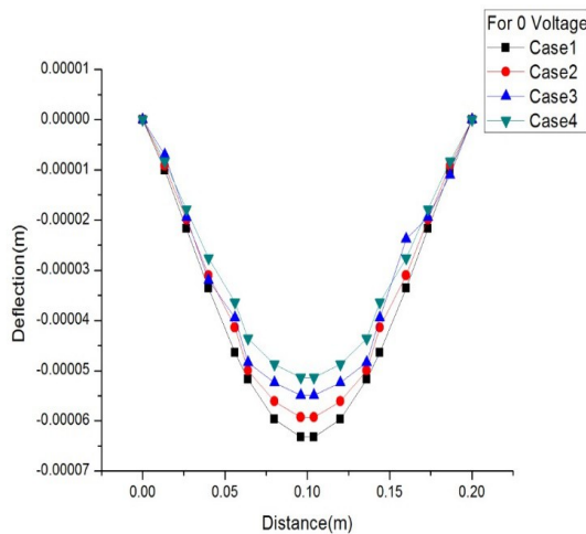
Fig 10: Centerline deflection for P=100N/m 2 , V=0 for different cases
