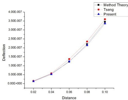
Fig 5: PVDF Bimorph Beam's Deflection (for a unit voltage) (m)
