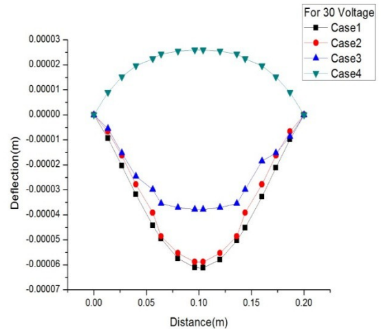
Fig 11: Centerline deflection for P=100N/m 2 , V=30 for different cases
