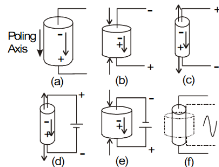
Fig 1.1: Piezoelectric effect
