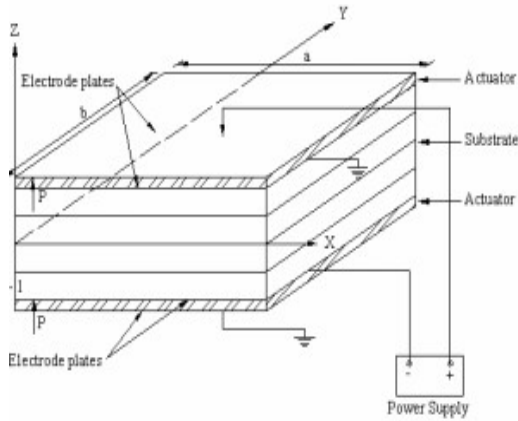
Fig2: Piezoelectric effect
