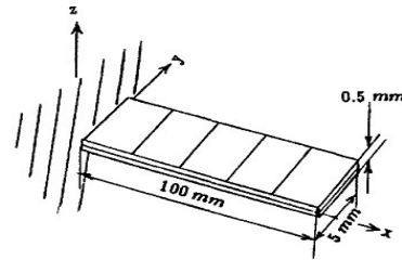
Fig 4: Piezoelectric PVDF BIMORPH BEAM.
