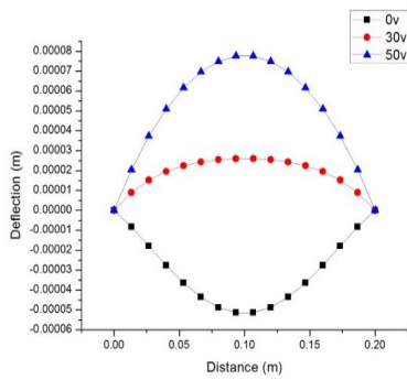
Fig 10: Centerline deflection of plate [p-45/45] as P=100N/m 2 , V=0,30,50
