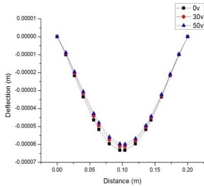
Fig 7: Centerline deflection of plate [p-45/45] as P=100N/m 2 , V=0,30,50
