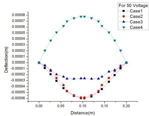
Fig 12: Centerline deflection for P=100N/m 2 , V=50 for number of cases
