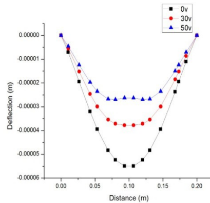
Fig 9: Centerline deflection of plate [p-45/45] as P=100N/m 2 , V=0,30,50
