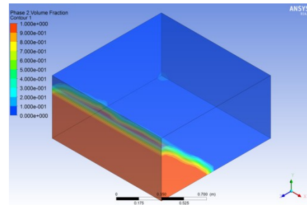
Fig.4.13 Volume portion of fluid at 1.8sec
