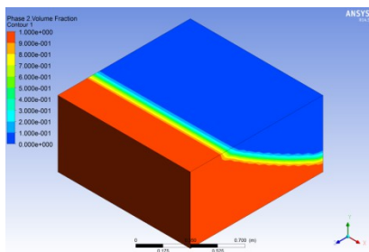
Fig.4.11 Volume fraction of fluid at 0.2sec
