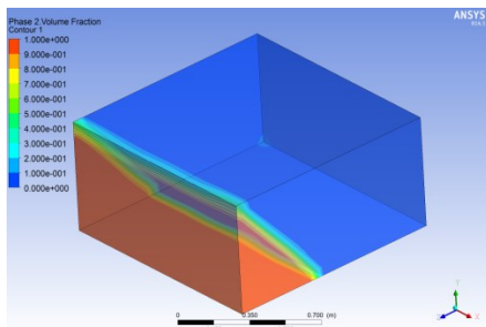
Fig.4.15 Volume portion of liquid at 3sec
