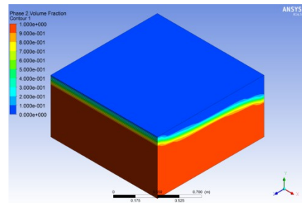
Fig.4.9 Volume portion of liquid at 0.01sec
